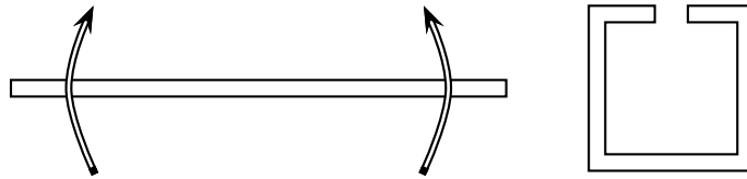
Figure 2.1: The square open loop resonator can be obtained by folding a straight open resonator.
