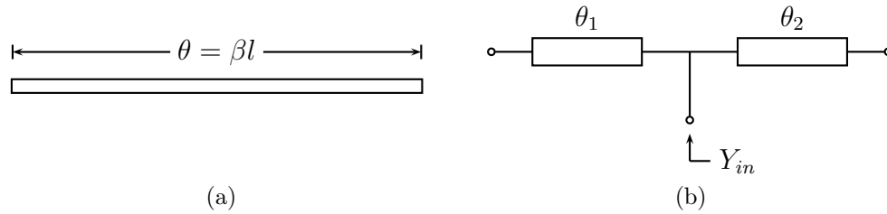
Figure 2.2: Microstrip open resonator. (a) Top view of a microstrip straight resonator. (b) Equivalent circuit used to calculate the input admittance from an arbitrary point within the length of the resonator.
