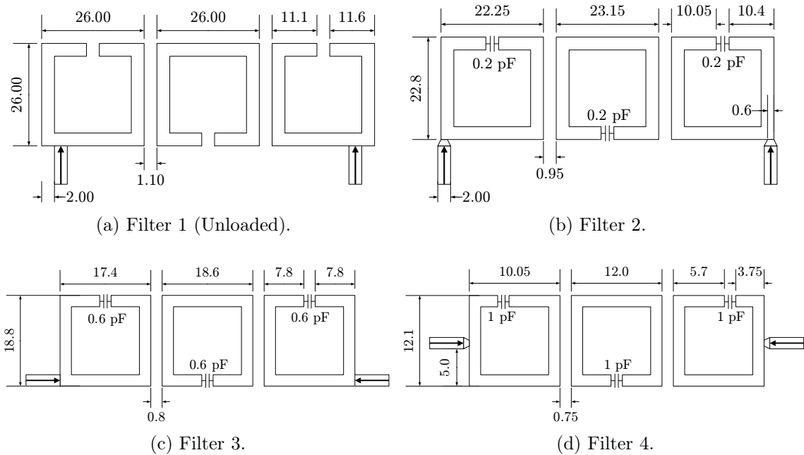
Figure 3.11: Layout of the four filter examples (units are mm).
