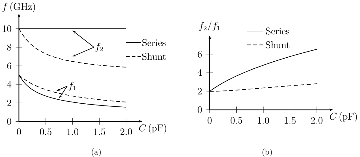
Figure 3.4: Resonant frequencies as a function of loading capacitance. (a) First and second resonant frequencies for series and shunt loading. (b) Ratio of the second to first resonant frequency for both cases.
