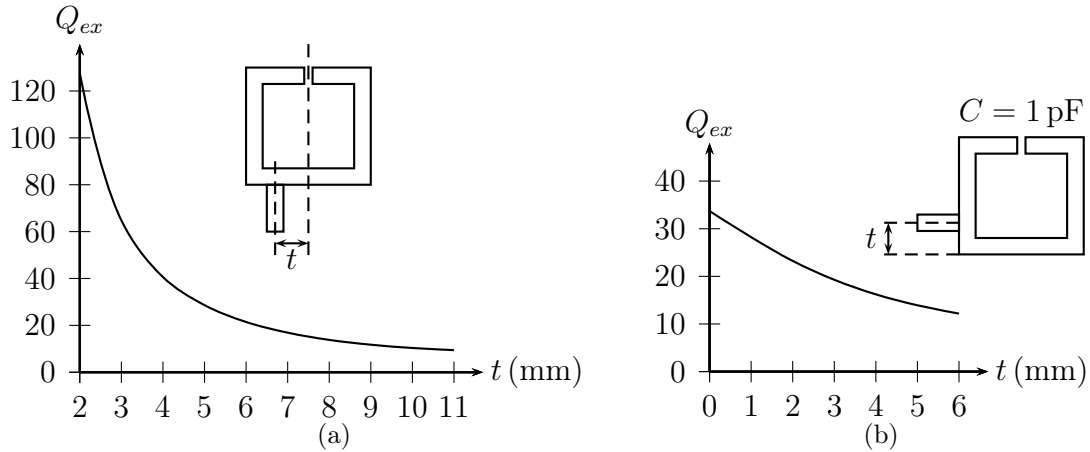
Figure 3.10: External quality factor of an: (a) unloaded resonator, and (b) a resonator loaded with C = 1 \text{ pF} (b).
